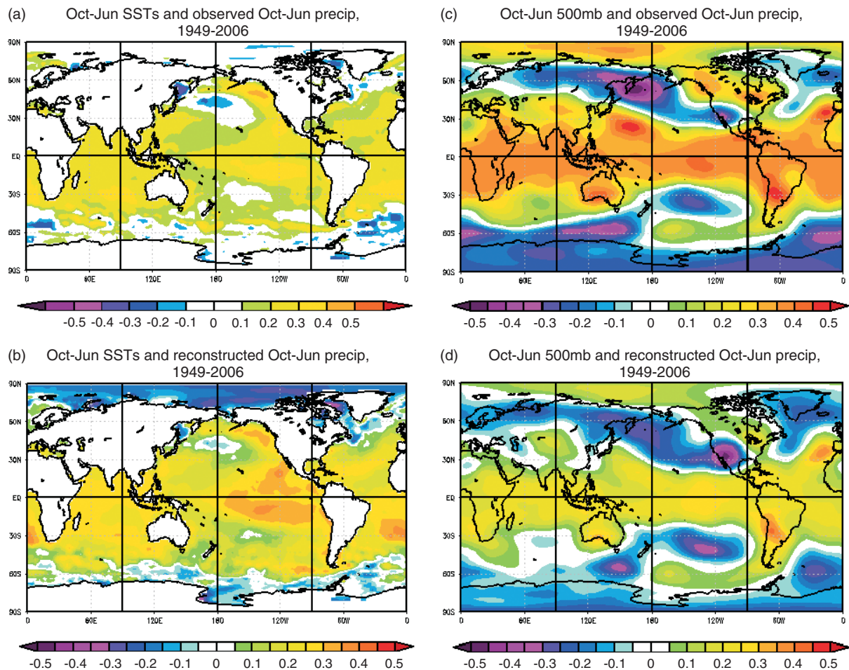
Figure 5. Correlations field maps, 1949–2006. (a) New Mexico Division 2 October–June precipitation and October–June SSTs. (b) New Mexico Division 2 reconstructed October–June precipitation and October–June SSTs. (c) New Mexico Division 2 October–June precipitation and October–June 500-mb geopotential heights. (d) New Mexico Division 2 reconstructed October–June precipitation and October–June 500-mb geopotential heights. Images provided by the NOAA/ESRL Physical Sciences Division, Boulder Colorado from their Website at http://www.esrl.noaa.gov/psd/ . This figure is available in colour online at wileyonlinelibrary.com/journal/joc
