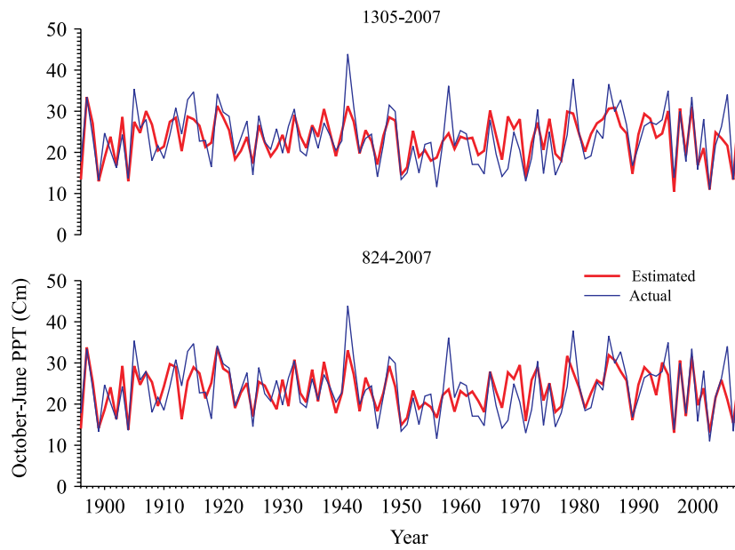
Figure 2. Comparison of actual and estimated October–June precipitation for the 1896–2005 period. This figure is available in colour online at wileyonlinelibrary.com/journal/joc
